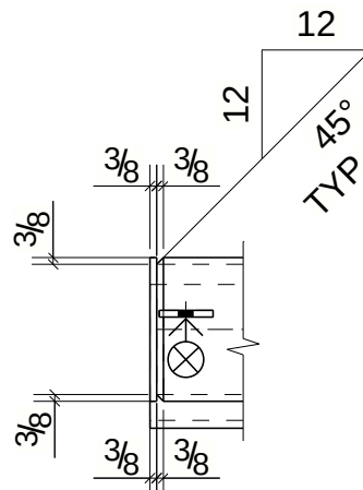
DETAIL A
